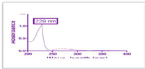
Figure 02:lambda max of Carteolol Hydrochloride.
