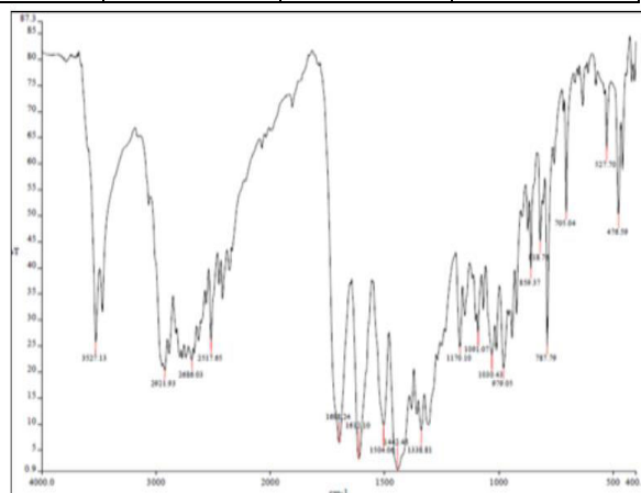
FIG. 03: IR SPECTRUM OF CARTEOLOL B. CALIBRATION CURVE OF CARTEOLOL
